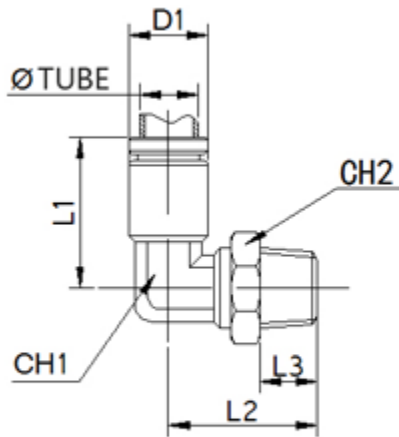
Dimensions of SPL 06-N02 90-Degree Elbow | Stainless Steel Push to Connect Fitting
